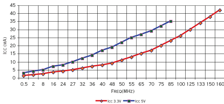
TYPICAL SUPPLY CURRENT ICC (MA) AT 3.3Vdc & 5.0Vdc NO LOAD
