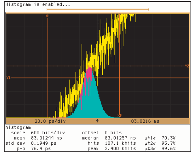
RMS jitter ( 1\sigma ): 8.19ps Peak-to-peak jitter: 76ps
