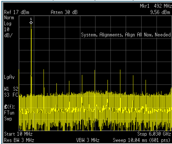
Output Power (+7.8 dBm)
