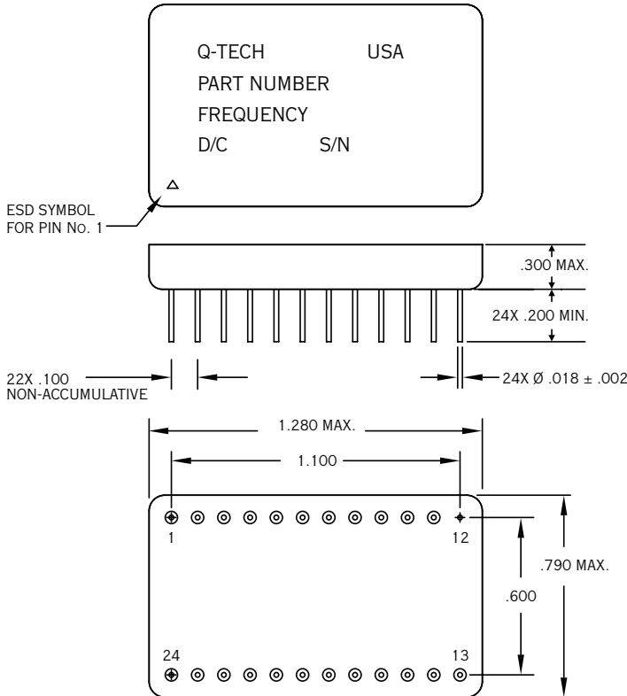
FIGURE 1 INTERFACE CONTROL DRAWING 24 Pin Double Dip
